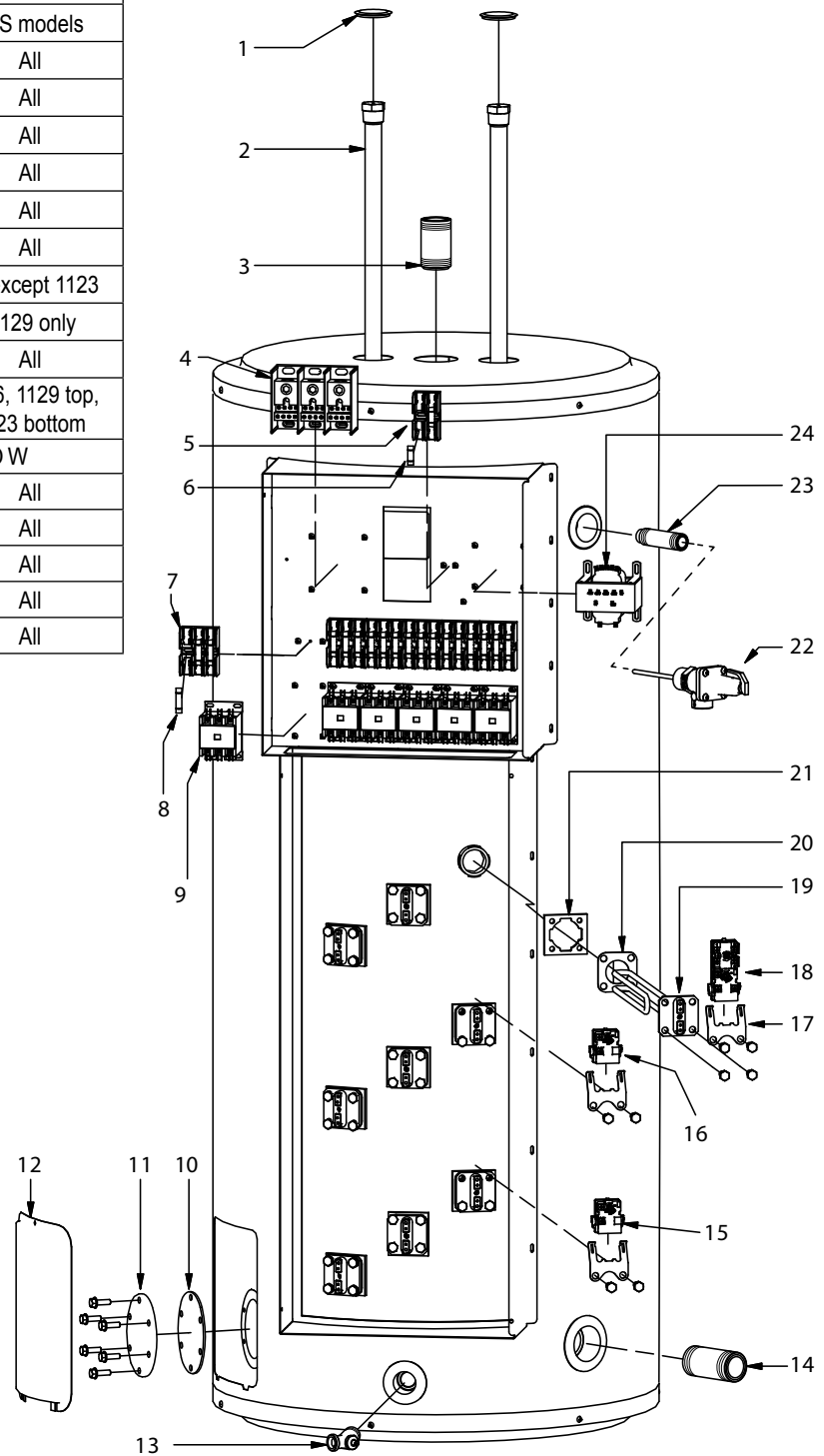
Illustration shows Model 112 with 9 elements
