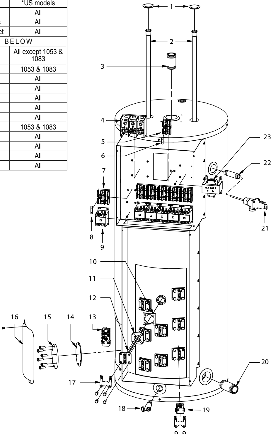
Illustration shows Model 108 with 9 elements
