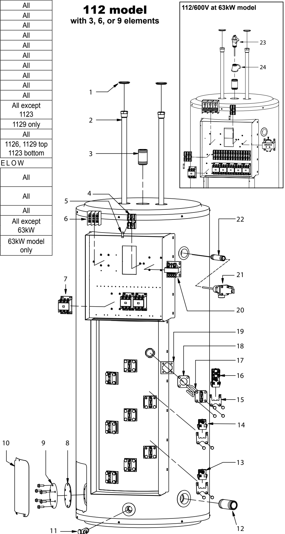
Illustration shows Model 112 with 9 elements
